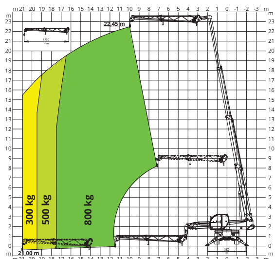
JIB WITH WINCH 2,000 kg
