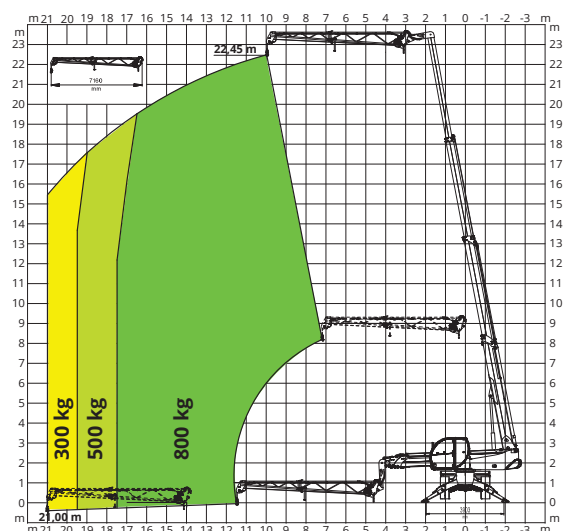
JIB WITH WINCH 800 kg
