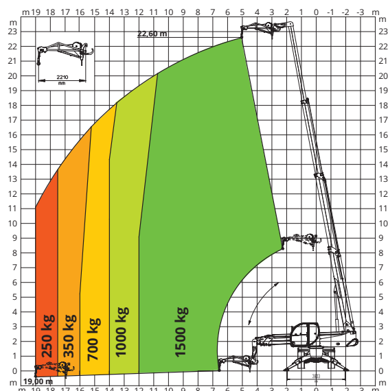
JIB WITH WINCH 1,500 kg
